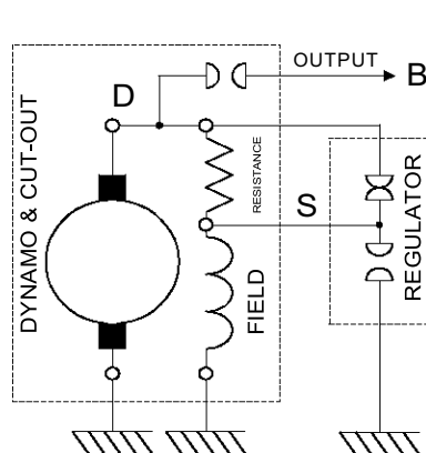
MILLER DVR 2 BRUSH (standard connections)
