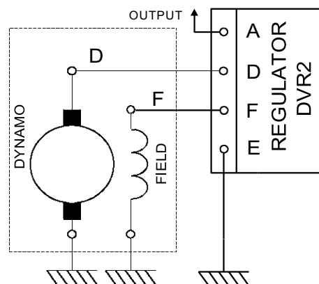
MILLER with DVR 2 (modified connections)
